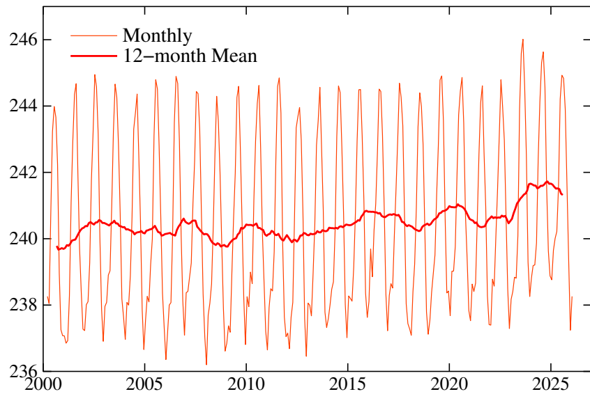
Global Emitted Thermal Radiation ( W/m^2 )
