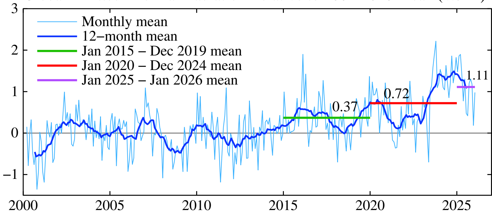
Global Emitted Thermal Radiation Relative to 2001-2010 Mean ( \text{W}/\text{m}^2 )
