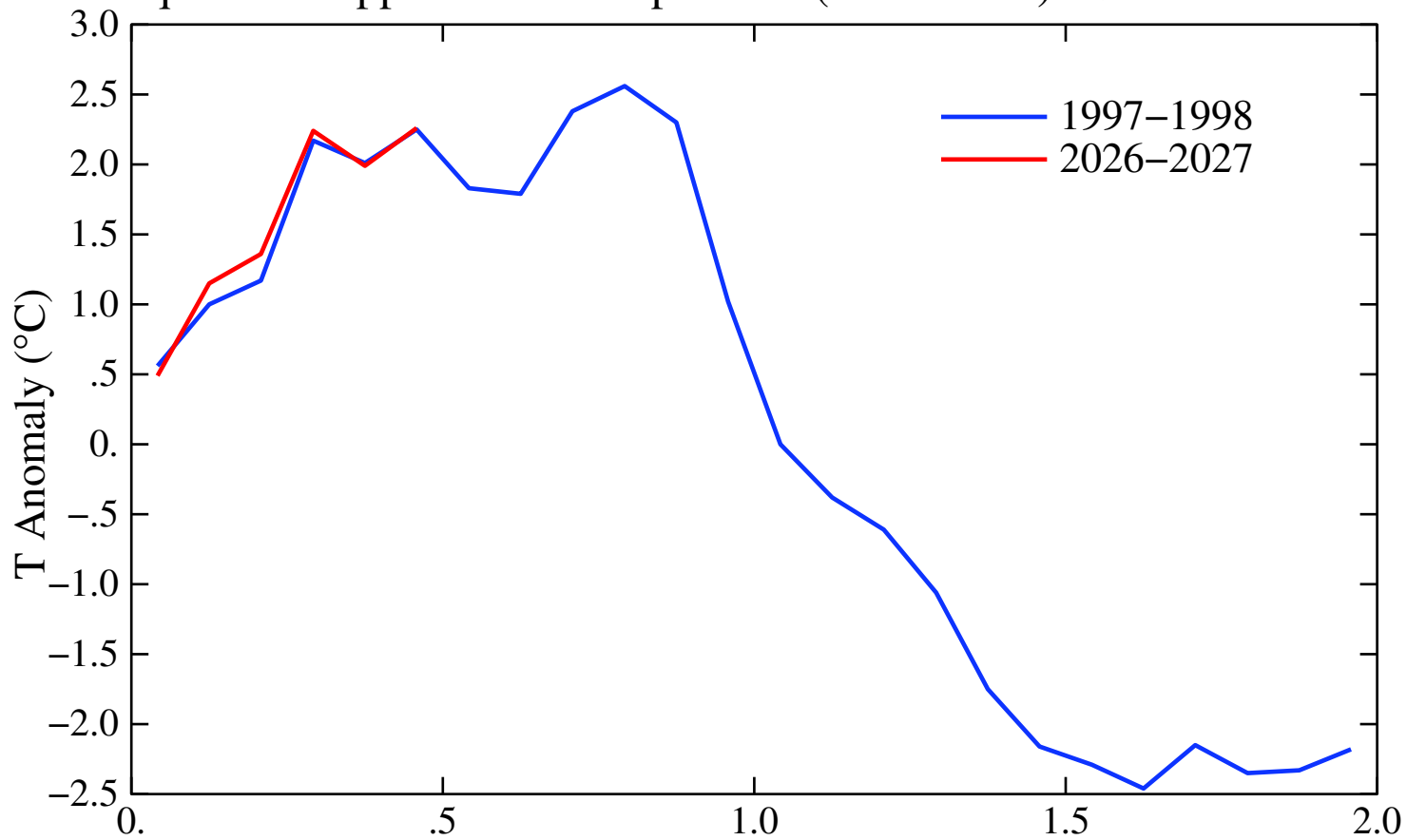
Equatorial Upper 300m Temperature (180–100W): 1981–2010 Base
