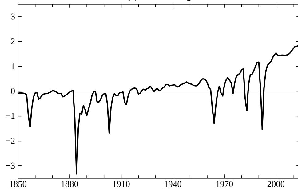
(b) Net Forcing
