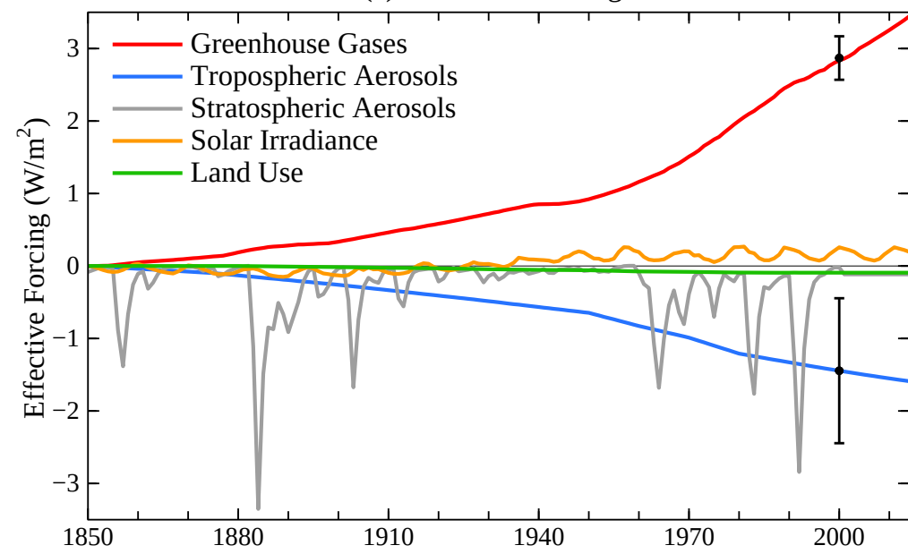
(a) Radiative Forcings
