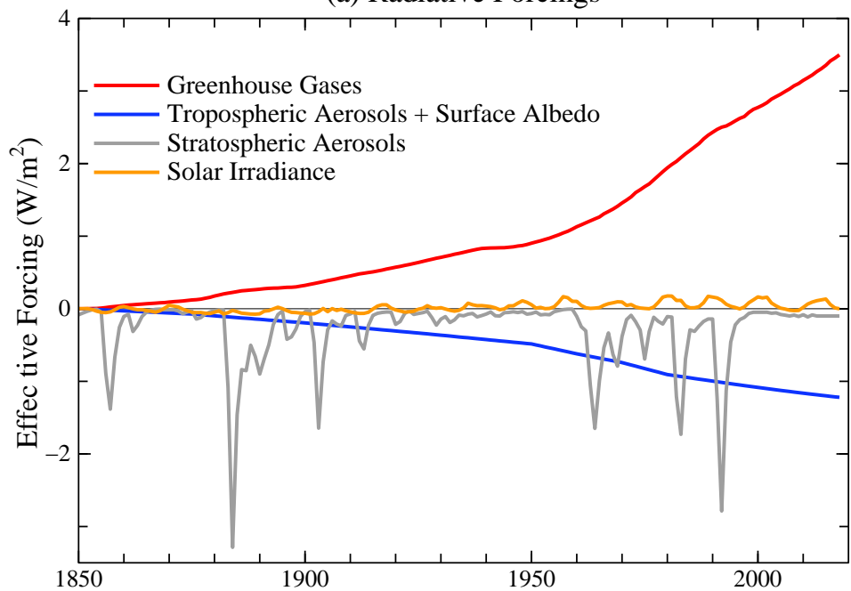
(a) Radiative Forcings
