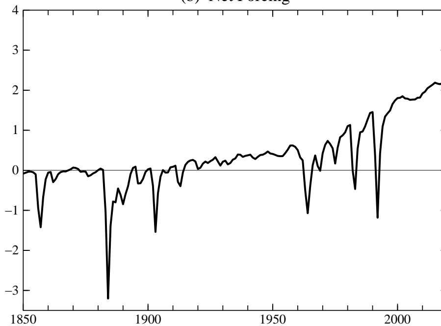
(b) Net Forcing
