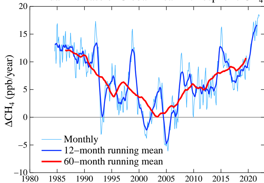
Annual Increase of Global Mean Atmospheric CH 4
