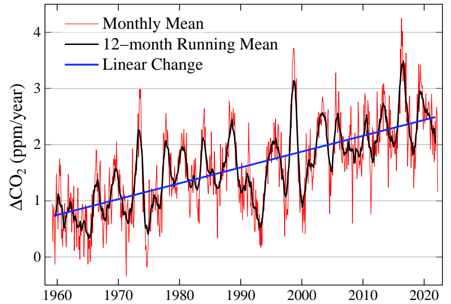
Annual Increase of Atmospheric CO 2 at Mauna Loa
