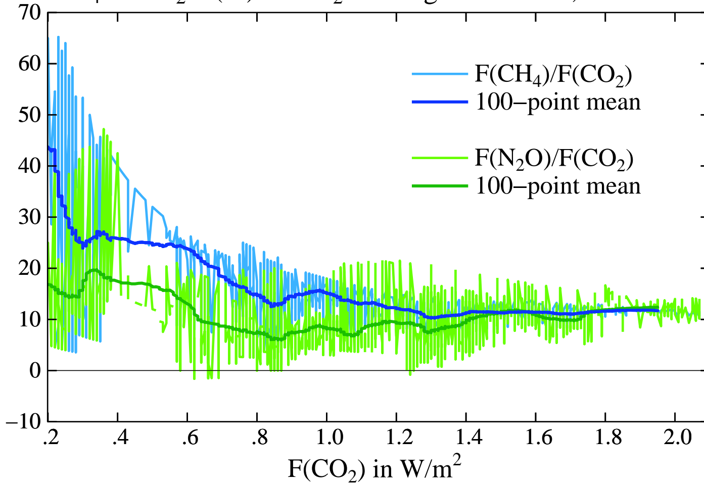
CH 4 and N 2 O (%) of CO 2 Forcing in Past 140,000 Years
