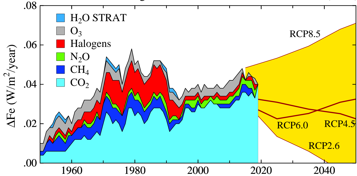
GHG Effective Forcing Growth Rate with RCPs from IPCC (2013)
