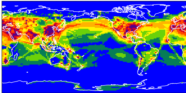
(a) Total sulfate
