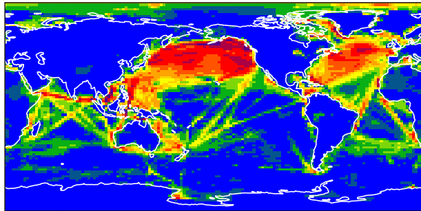
(b) Percent of total sulfate from shipping
