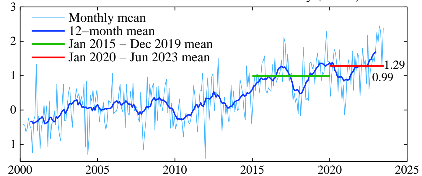
Global Absorbed Solar Radiation Anomaly ( \text{W/m}^2 )
