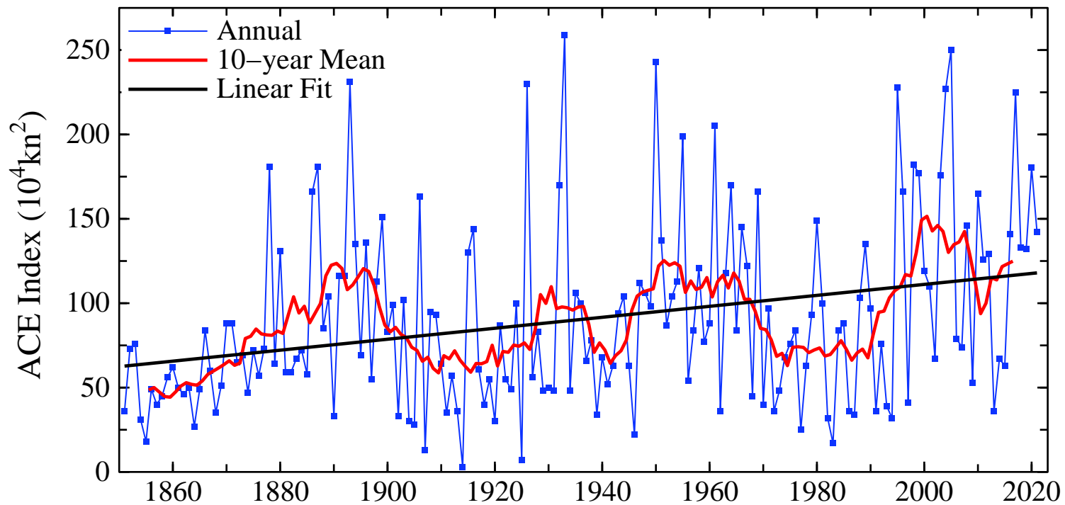
Accumulated Cyclone Energy: Atlantic Basin
