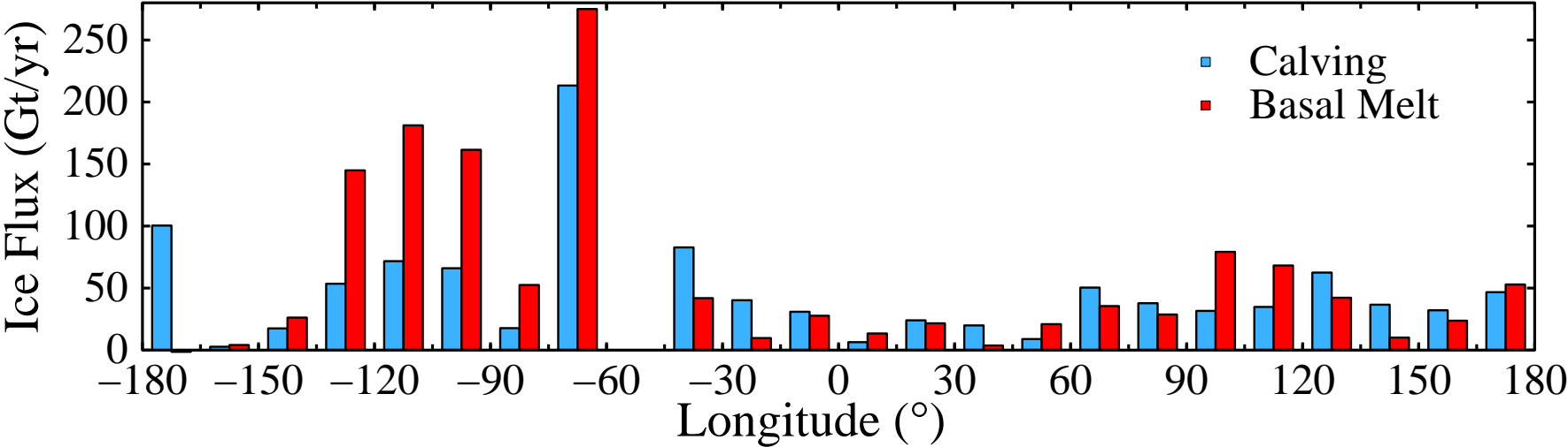
Freshwater Production by Calving and Basal Melt
