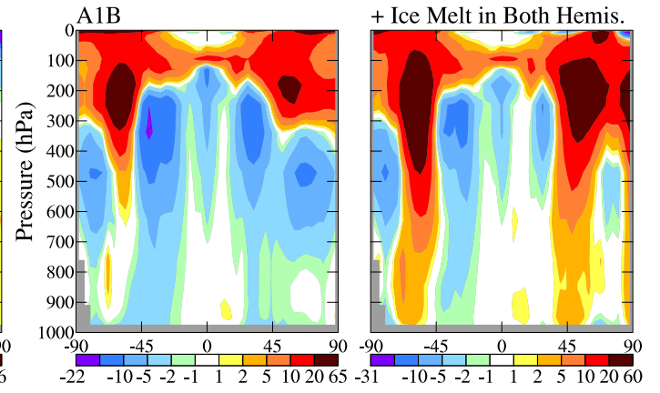
Eddy Kinetic Energy Anomaly ( m^2/s^2 )
