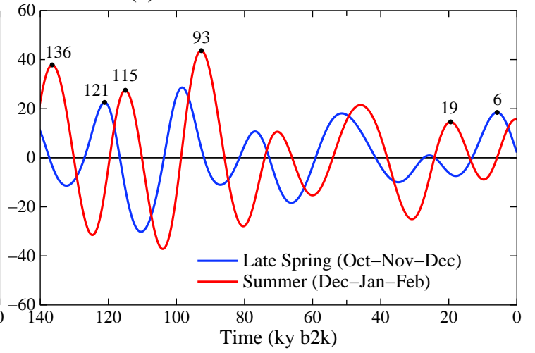
(b) Insolation Anomalies at 60°S
