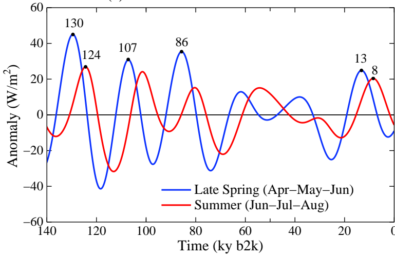
(a) Insolation Anomalies at 60°N
