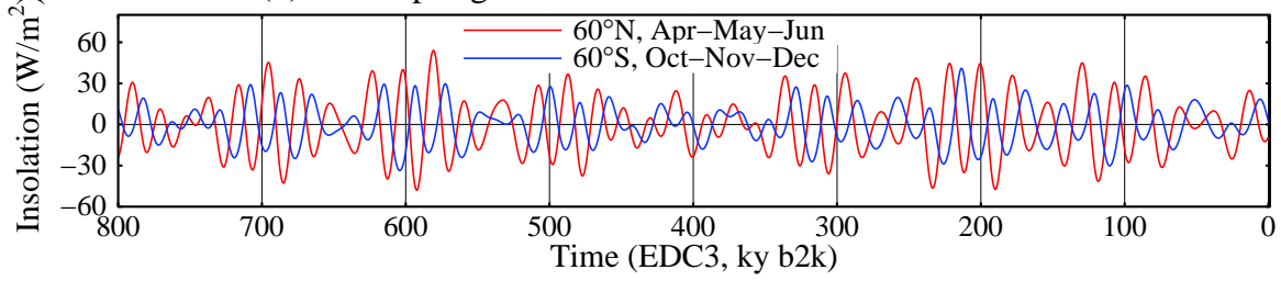
(b) Late Spring Insolation Anomalies at 60°N and 60°S
