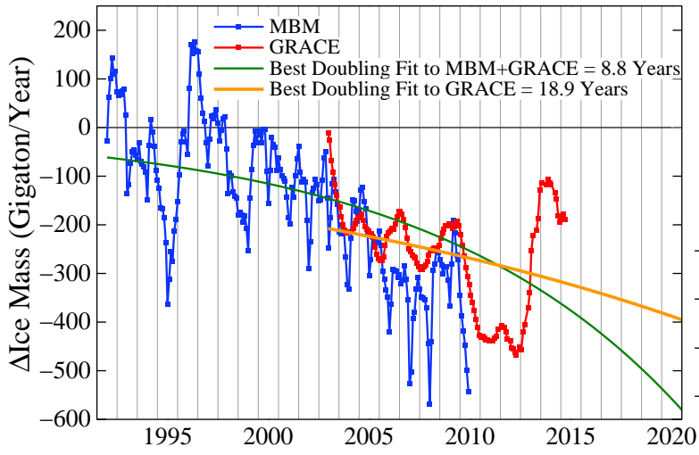
(a) Greenland Ice Mass Change Rate
