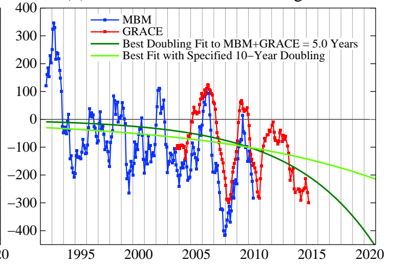
(b) Antarctica Ice Mass Change Rate
