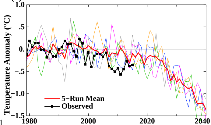
(b) West Antarctic SST with 1979-2000 Base Period
