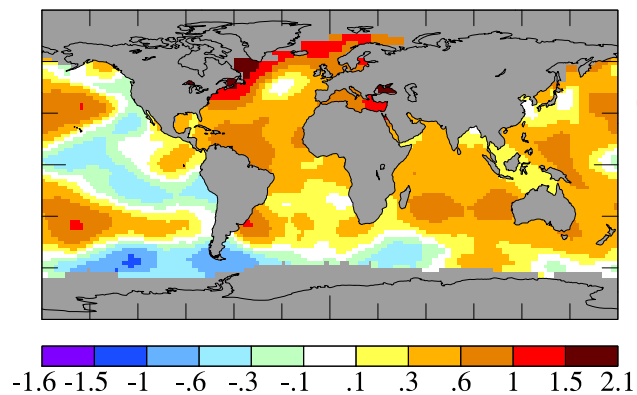
(a) SST Change in Past 25 Years ( ^{\circ}\text{C} ) 1990-2015
