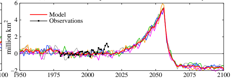
(b) Southern Hemispheric Mean Sea Ice Area Anomaly
