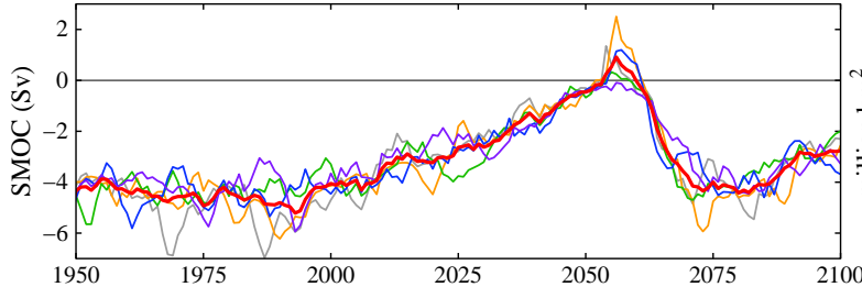
(a) SMOC at 72°S, 2.1 km Depth
