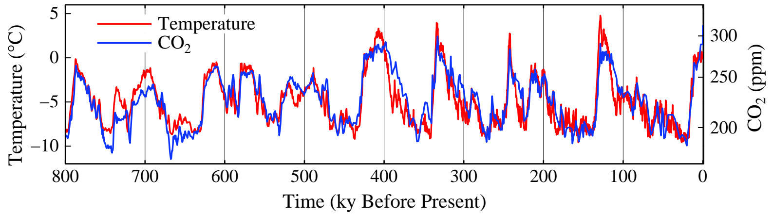
Atmospheric CO 2 Amount and Antarctic Temperature Change
