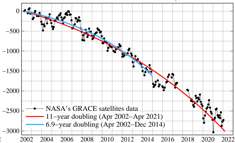
(b) Antarctica Ice Mass Change
