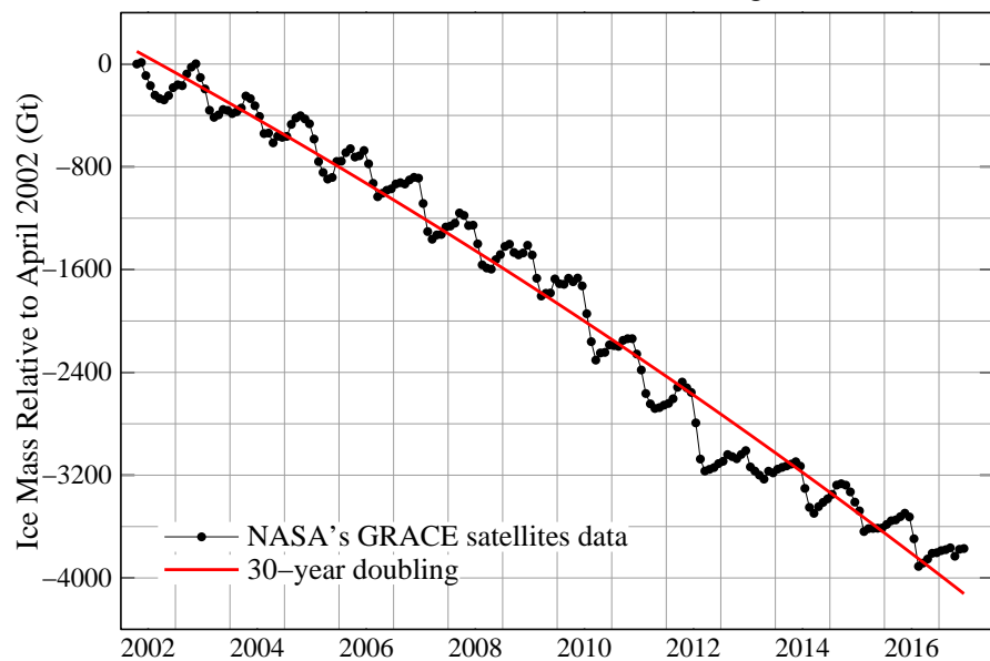
(a) Greenland Ice Mass Change
