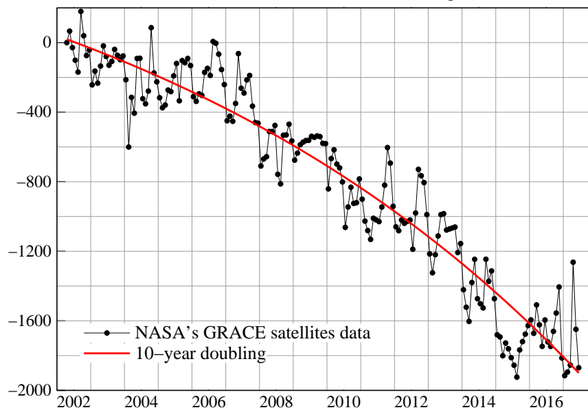
(b) Antarctica Ice Mass Change
