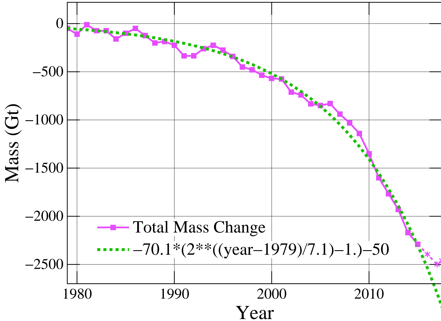
Rignot et al. (2019) Fig. 3A West Antarctica Ice Mass
