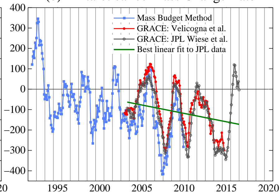
(b) Antarctica Ice Mass Change Rate
