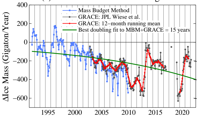
(a) Greenland Ice Mass Change Rate
