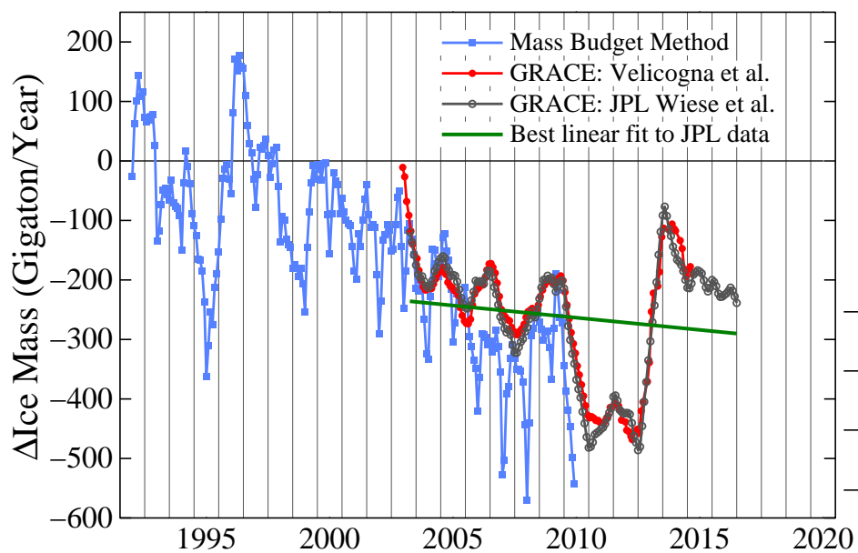
(a) Greenland Ice Mass Change Rate
