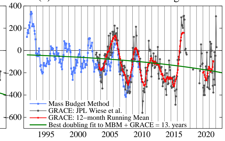
(b) Antarctica Ice Mass Change Rate
