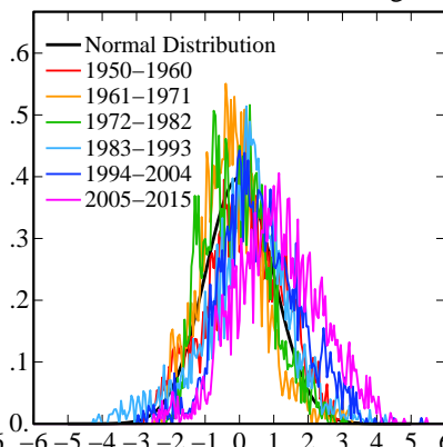
United States, Jun-Jul-Aug
