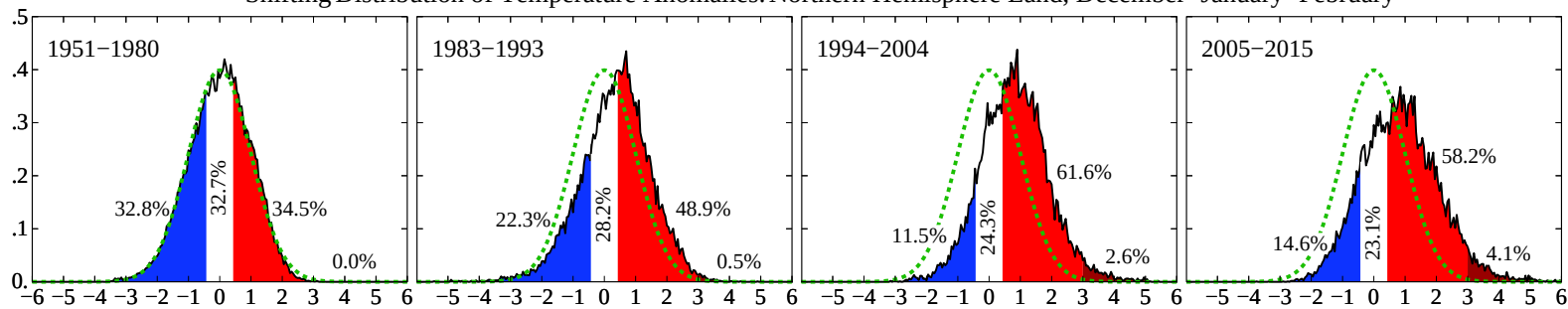
Shifting Distribution of Temperature Anomalies: Northern Hemisphere Land, December–January–February
