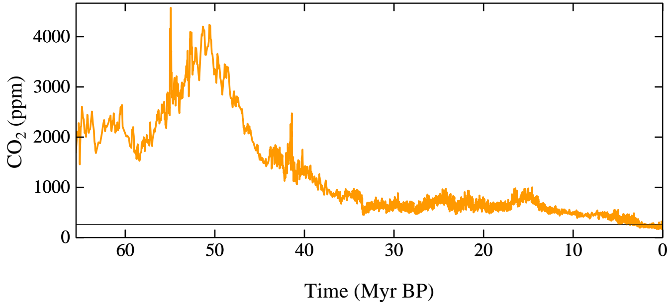
Implied CO 2 for State Independent Sensitivity
