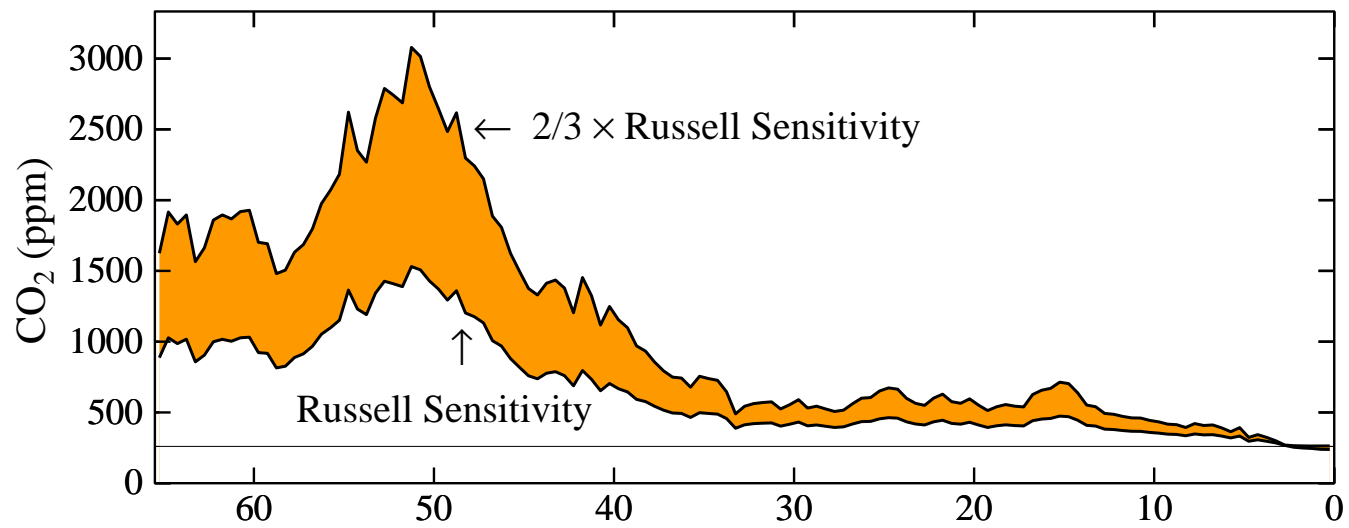
Implied CO 2 for State Dependent Sensitivity
