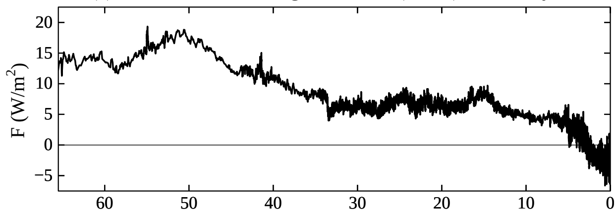
(b) Solar and Albedo Forcings
