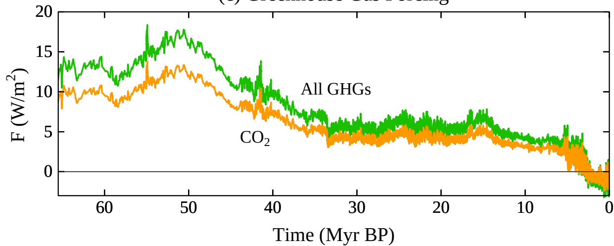
(c) Greenhouse Gas Forcing
