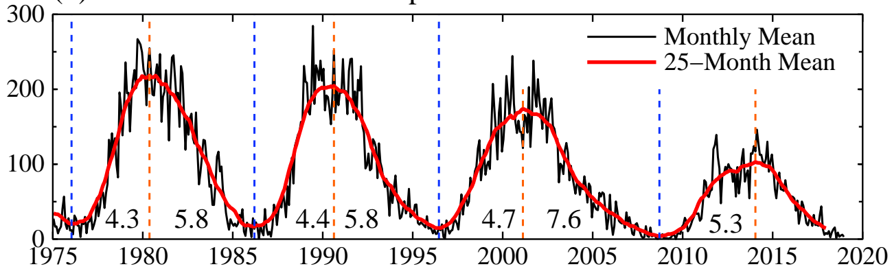
(b) Sunspot Numbers
