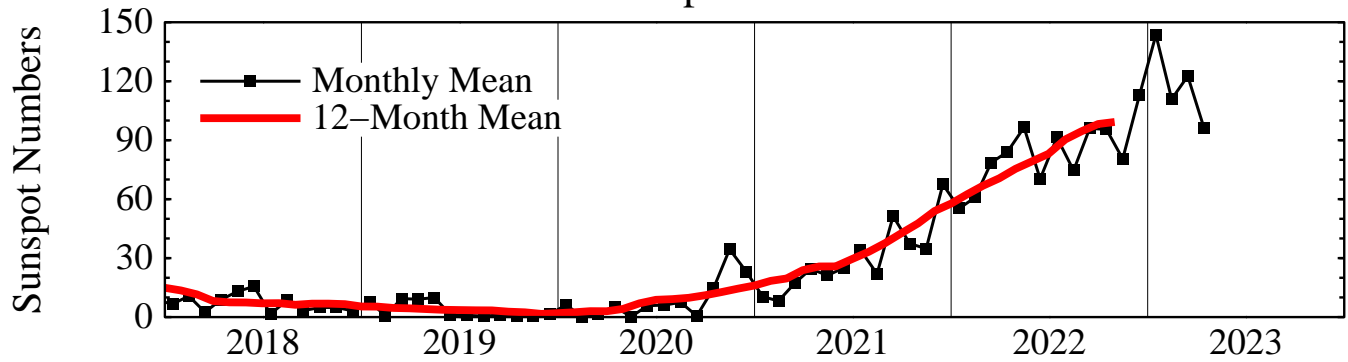
Sunspot Numbers
