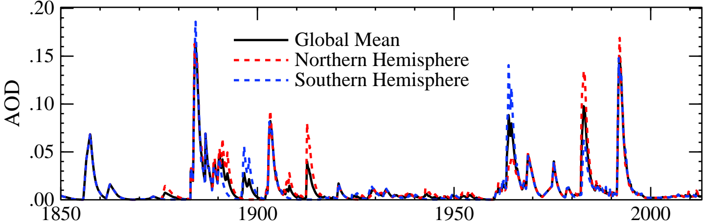
Monthly-Mean Stratospheric Aerosol Optical Depth at 550 nm
