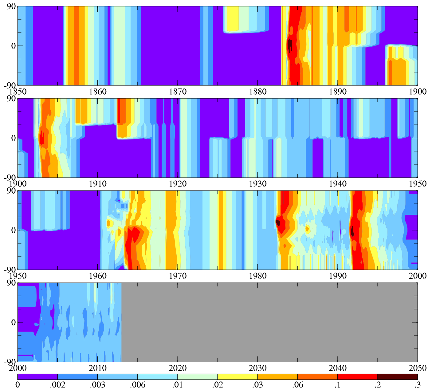
Zonal Mean Stratospheric Aerosol Optical Depth at 550 nm
