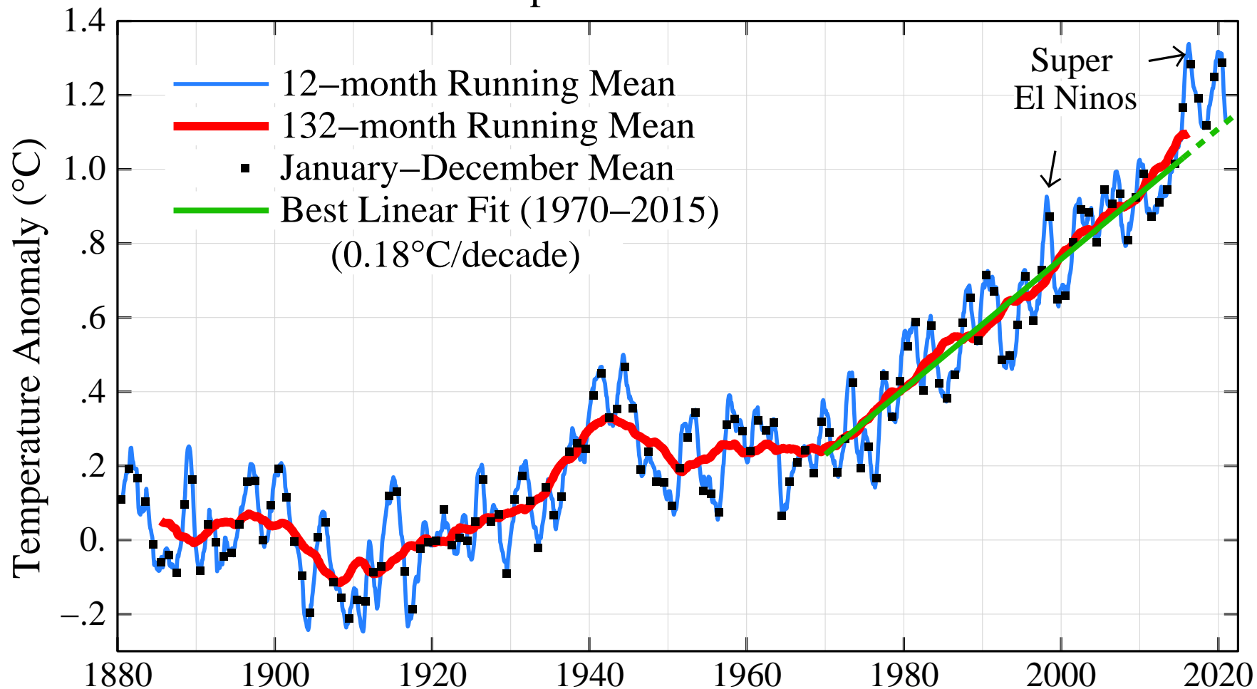
Global Surface Temperature Relative to 1880–1920 Mean
