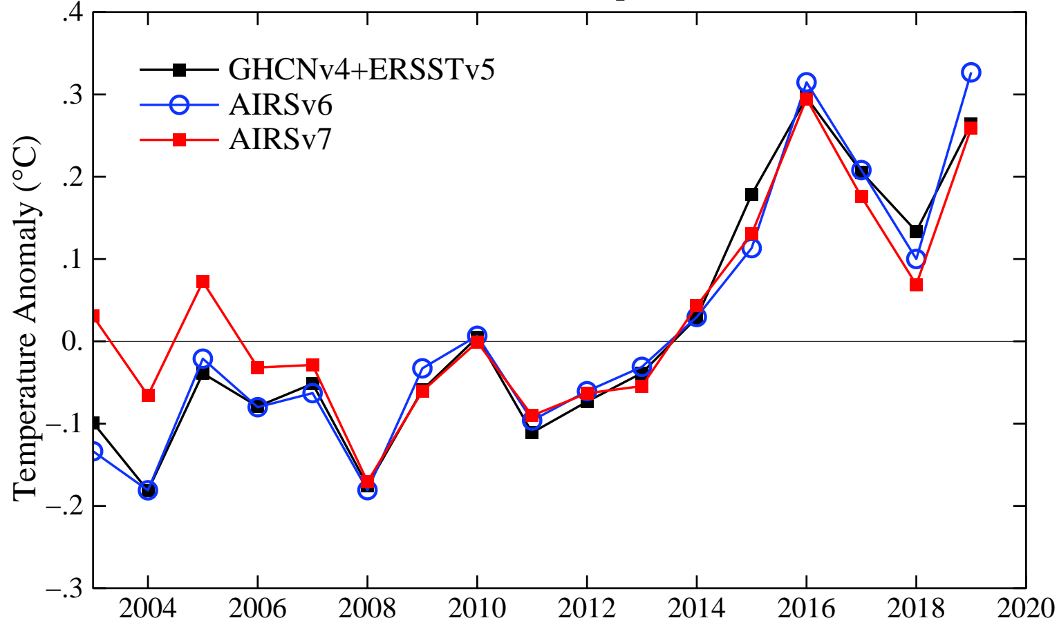
Annual Global Mean Surface Temperature: 2007–2016 Base
