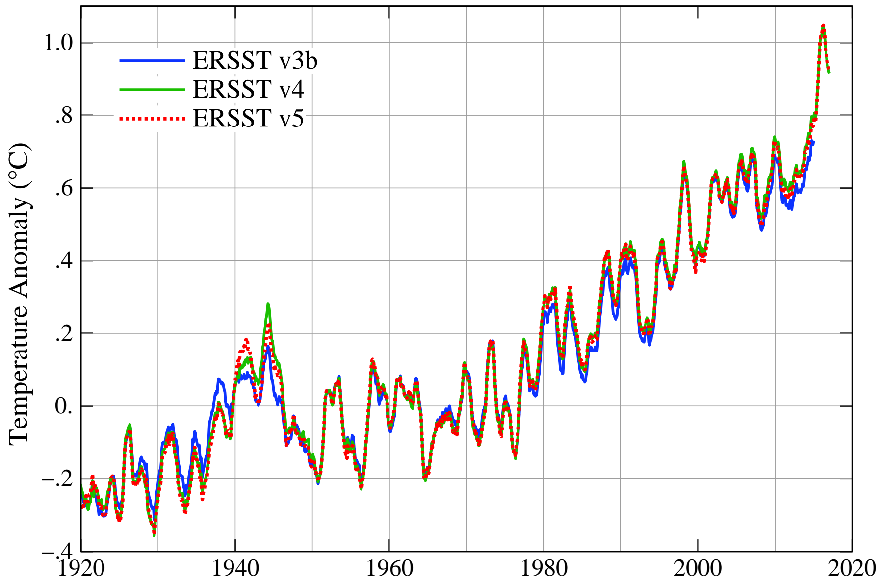
Global Surface Temperature: 12-month running means
