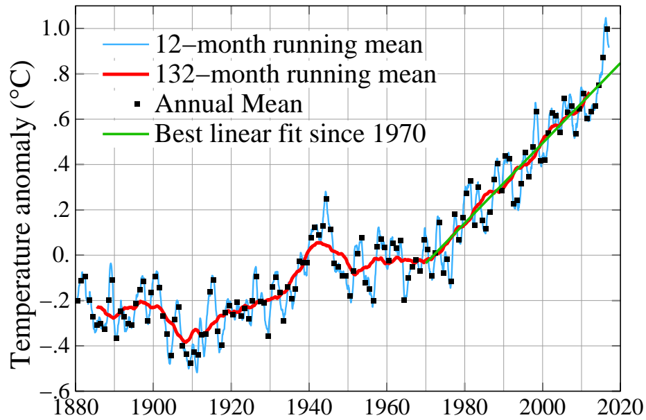
Global Surface Temperature with ERSSTv4
