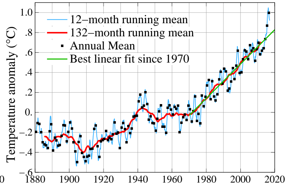
Global Surface Temperature with ERSSTv5
