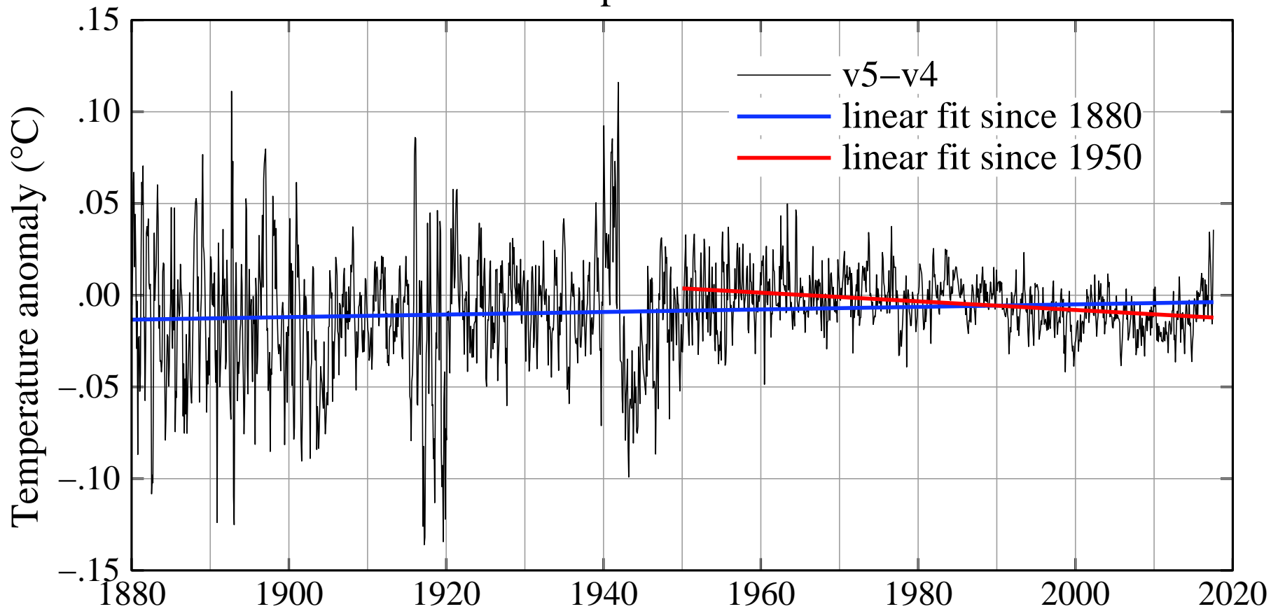
Global Mean Surface Temperature Difference: ERSST v5 – v4
