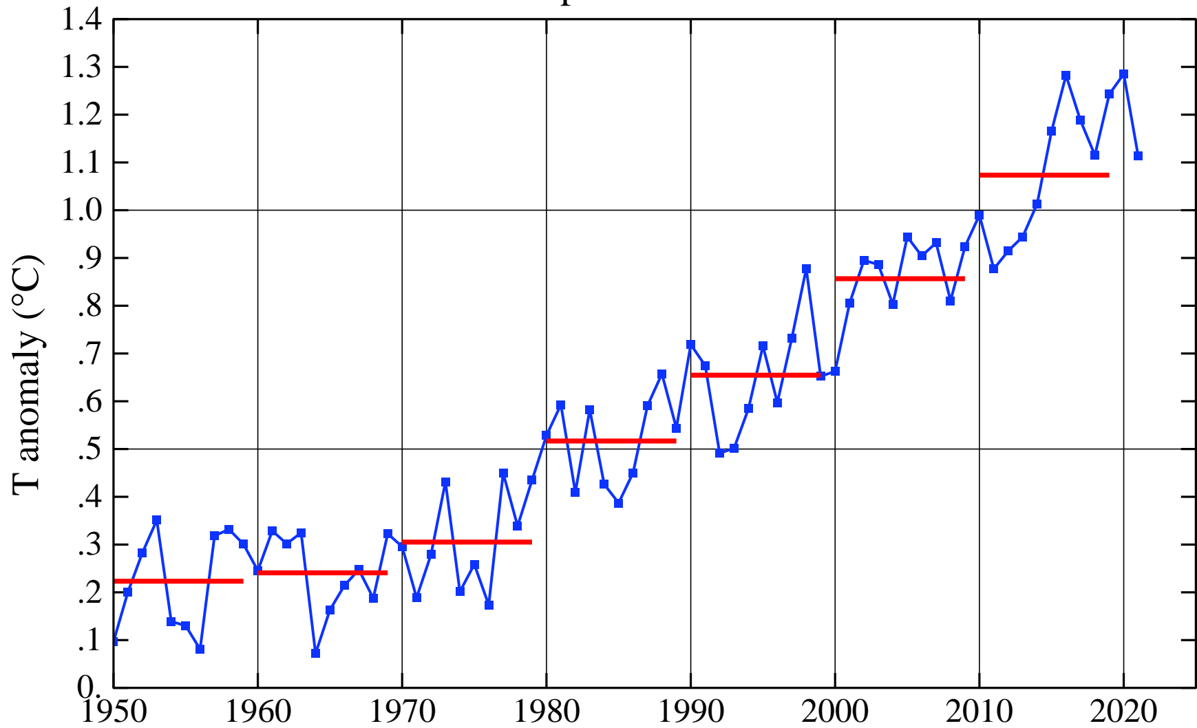
Annual Mean Global Temperature Relative to 1880–1920 Mean
