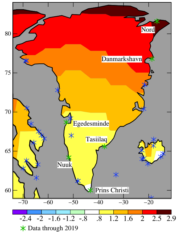
1950-2019 Linear Trend Temperature Change (°C) Meteorological Stations
