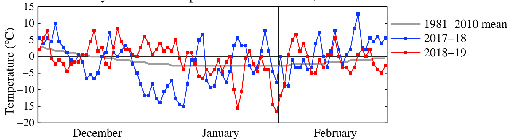
Daily Minimum Temperature at Central Park, NYC
