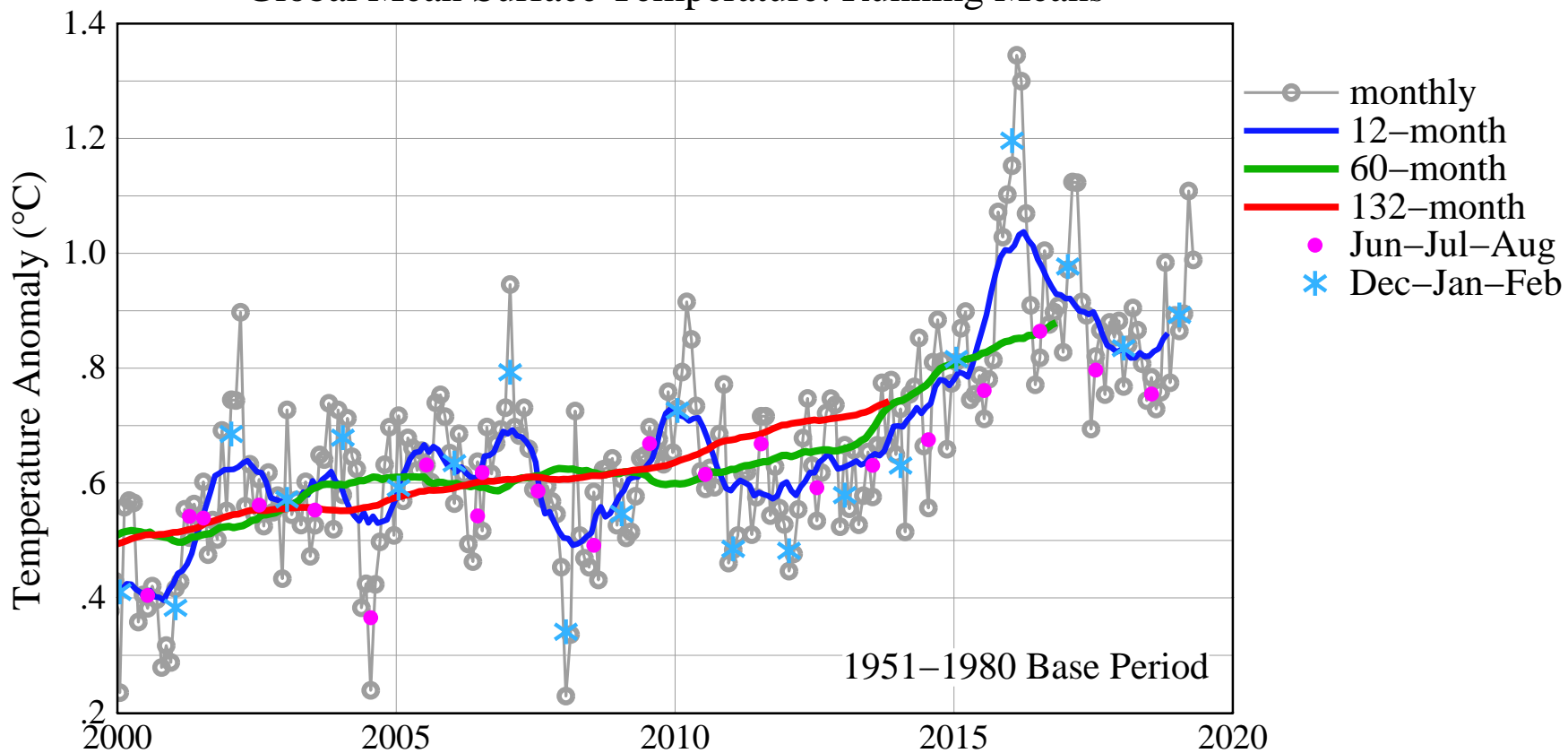
Global Mean Surface Temperature: Running Means
