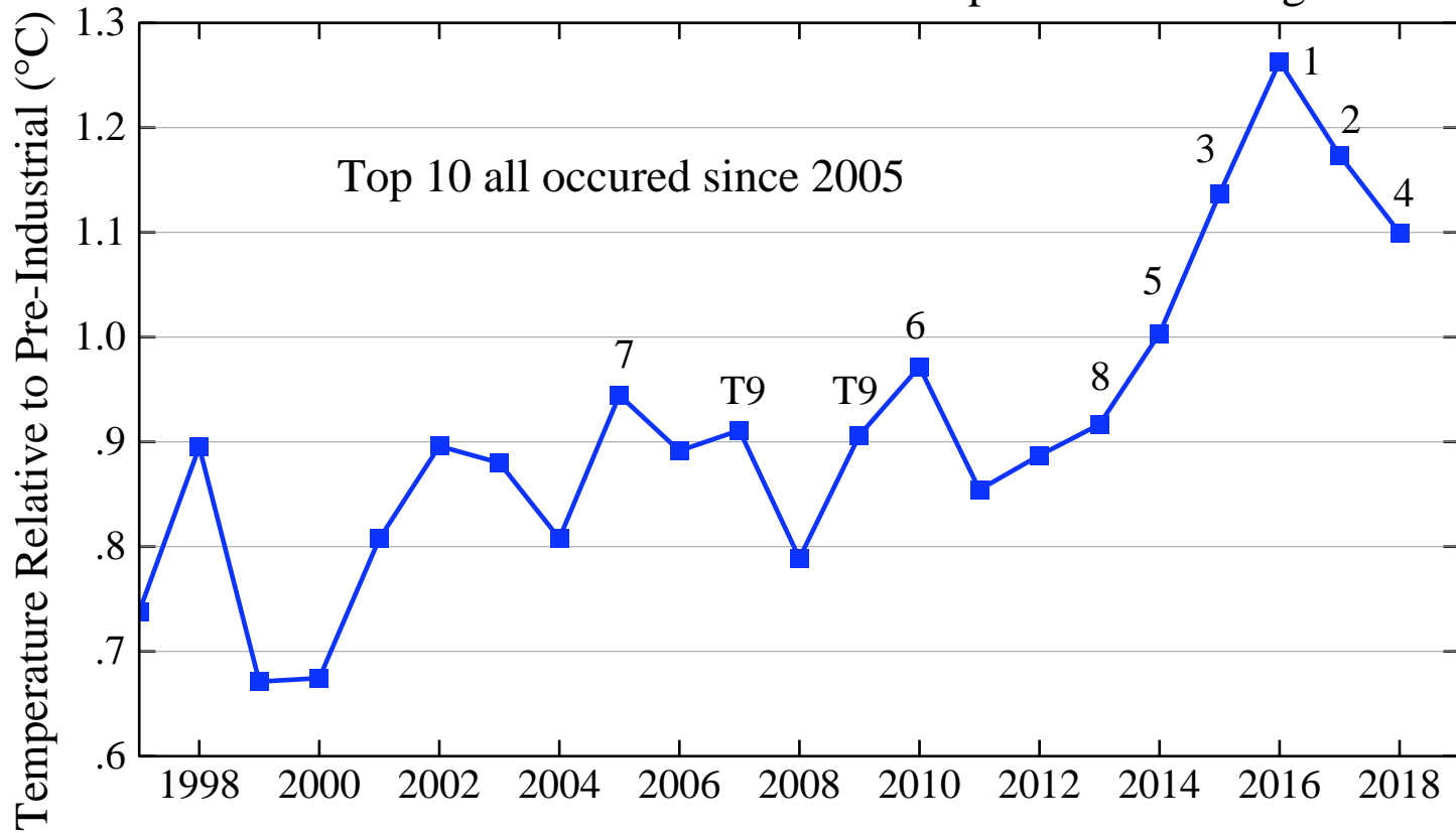
Annual Global Mean Surface Temperature Ranking
