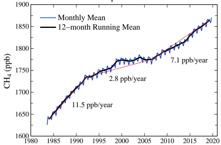
Global Mean Atmospheric Methane Abundance
