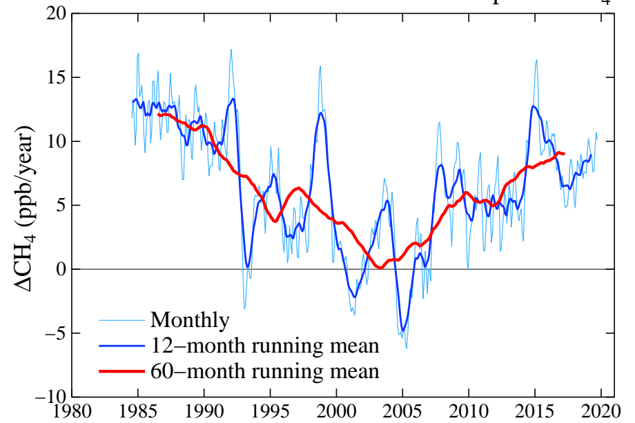
Annual Increase of Global Mean Atmospheric CH 4
