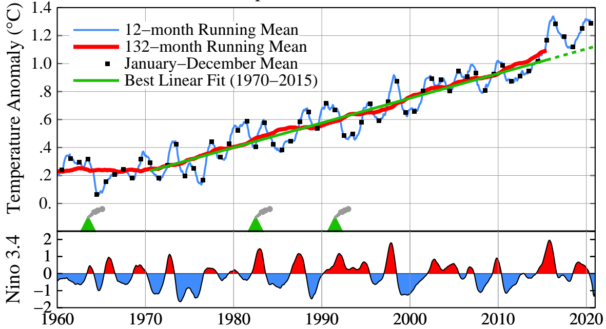
Global Surface Temperature Relative to 1880–1920 Mean
