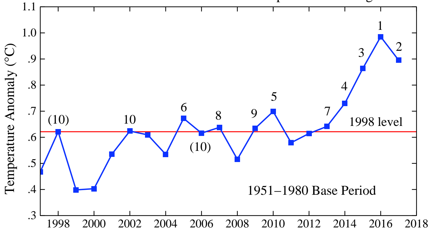
Annual Global Mean Surface Temperature Ranking
