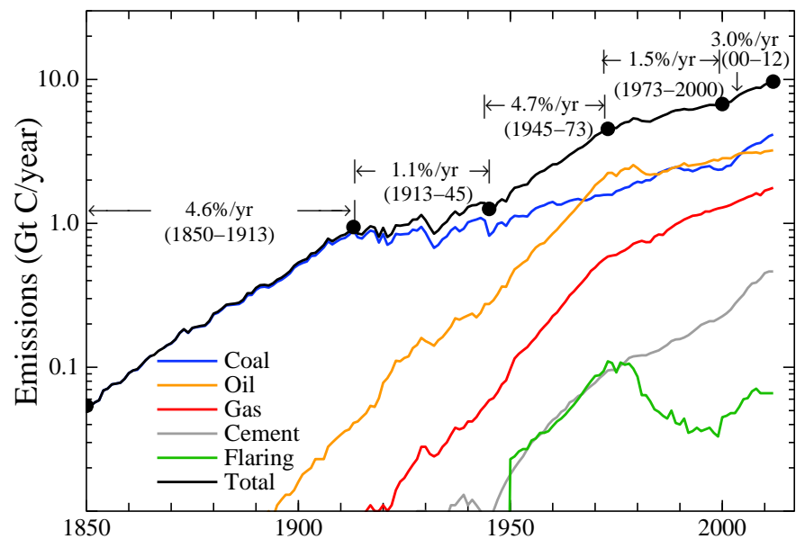
A Global Fossil-Fuel CO 2 Annual Emissions
