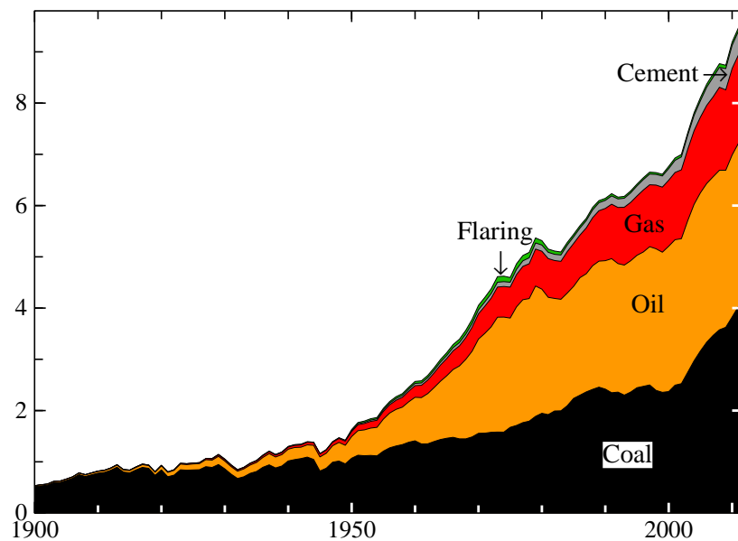
B Global Fossil-Fuel CO 2 Annual Emissions
