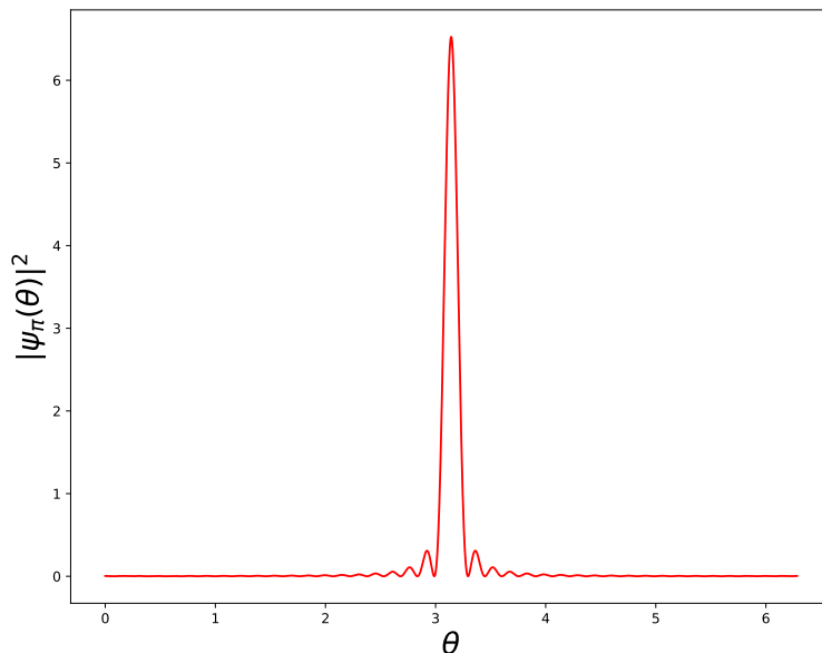
Figure 2: Plot of the modulus squared of the localized wave function \psi_\pi(\theta) for the case j = 10 . The x axis is shown in radians.
