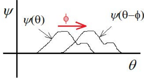
Figure 1: Diagram showing the original function \psi(\theta) and the new function \psi(\theta - \phi) obtained after the function \psi(\theta) is rotated through +\phi about the \hat{z} direction
