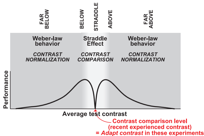
Figure 5. Idealized version of results in second-order orientation-identification experiments (e.g., Figure 4). We have suggested that the drop in performance in the center—the straddle effect—is the result of a shifting, rectifying contrast-comparison process (a process previously nicknamed “Buffy”). The contrast-comparison level shifts to equal the recently experienced contrast (which in these experiments is the adapt contrast). We have also suggested that the drops in performance at the two ends (which obey Weber’s law) are the result of a contrast-normalization process. (Later in this article we show similar results for first-order experiments.)
