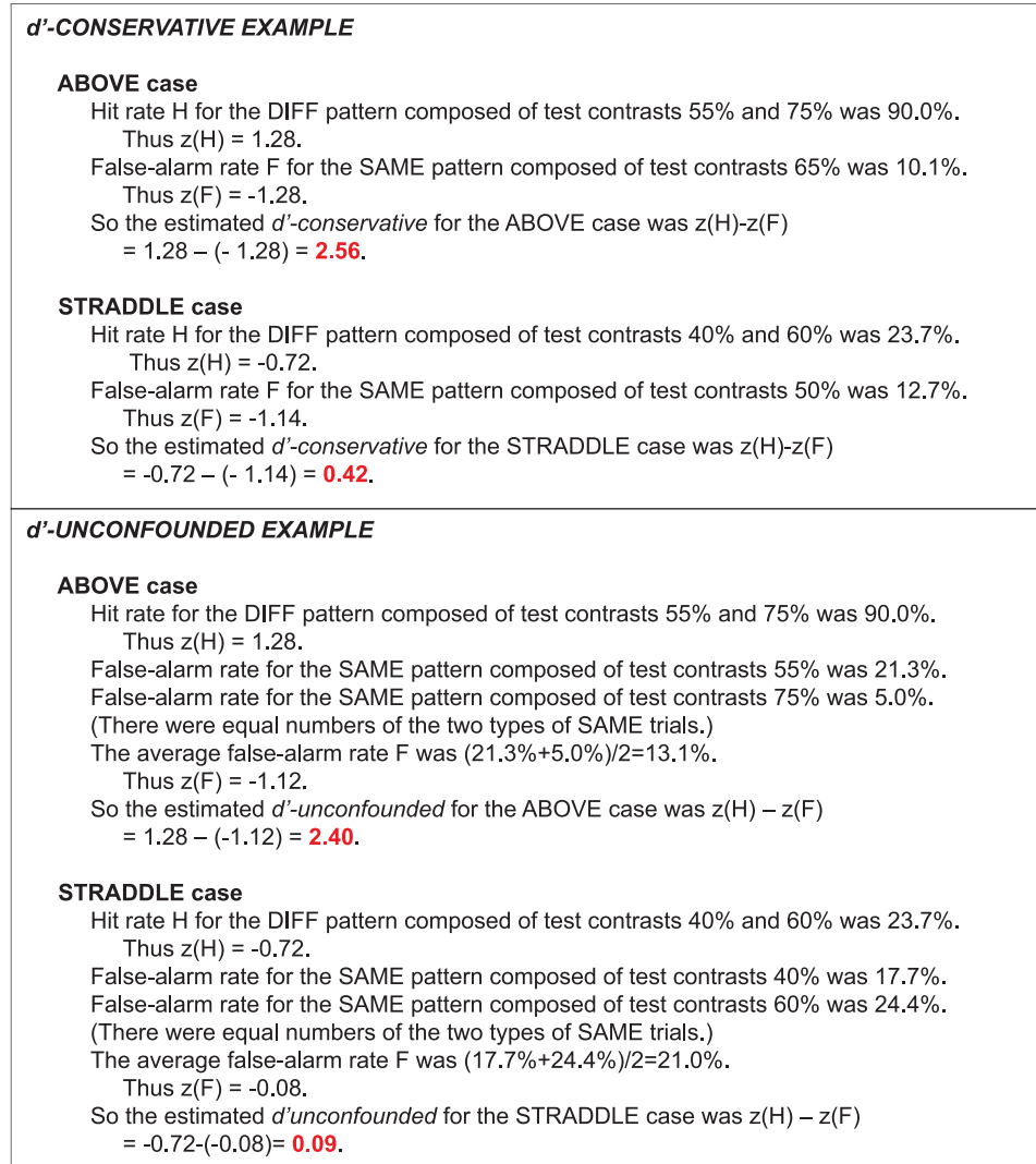
Figure B2. Step-by-step examples of calculating d' -conservative and d' -unconfounded.
