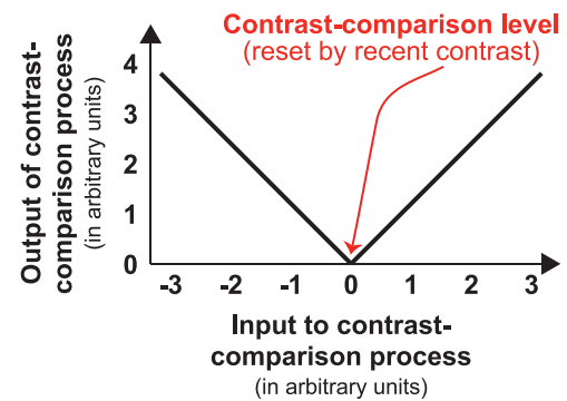
Figure 6. Diagram of the action of a shifting, rectifying contrast-comparison process. The input to this process—on the horizontal axis—reflects the local contrast at each position in the visual field, perhaps something like the size of a single Gabor patch. This input is compared to a comparison level indicated by the red arrow. The comparison level adapts over time to equal the recently experienced contrast. The output from this process is an unsigned measure of the difference between the current contrast and the recent average contrast. A more complete picture of the input/output functions from the contrast-comparison process is published in Graham (2011, figure 17).
