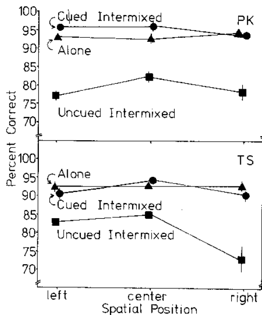
Figure 2. Results from the spatial-position uncertainty experiments. The position of the grating is shown on the horizontal axis. All other conventions are the same as in Figure 1.
