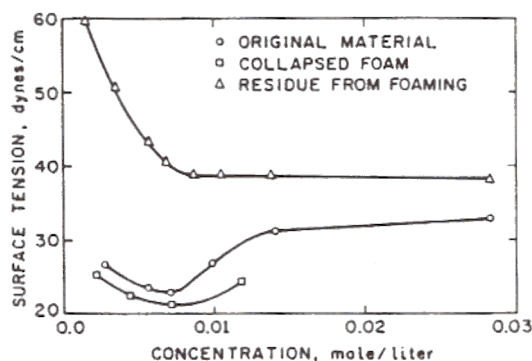
Figure 3. Surface tension of impure and foam-fractionated sodium lauryl sulfate solutions (19) .
