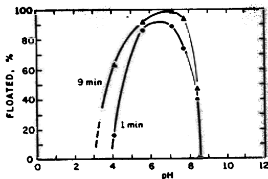
Figure 15. The effect of pH on the microflotation of E. coli . Initial concentration of organisms, 7.2 \times 10^8 /ml.; gas flow rate, 10.8 ml./min; collector concentration (lauric acid), 40 mg./l.; alcohol frother dose, 1 ml./400 ml; \text{Al}_2(\text{SO}_4)_3 \cdot 18\text{H}_2\text{O} concentration, 100 mg/l. (57) .
