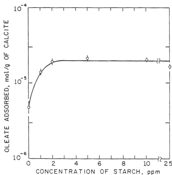
Figure 12 Adsorption density of oleate on calcite at natural pH 9.6–9.8 as a function of starch added prior to the oleate addition; vertical lines indicate the standard deviation in adsorption density due to the variation in the scintillation counting (49) .
