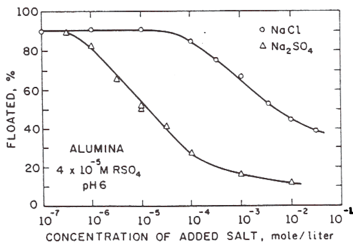
Figure 9. The depression of flotation of alumina by NaCl and Na 2 SO 4 with sodium dodecylsulphate as the collector at pH 6 (41) .
