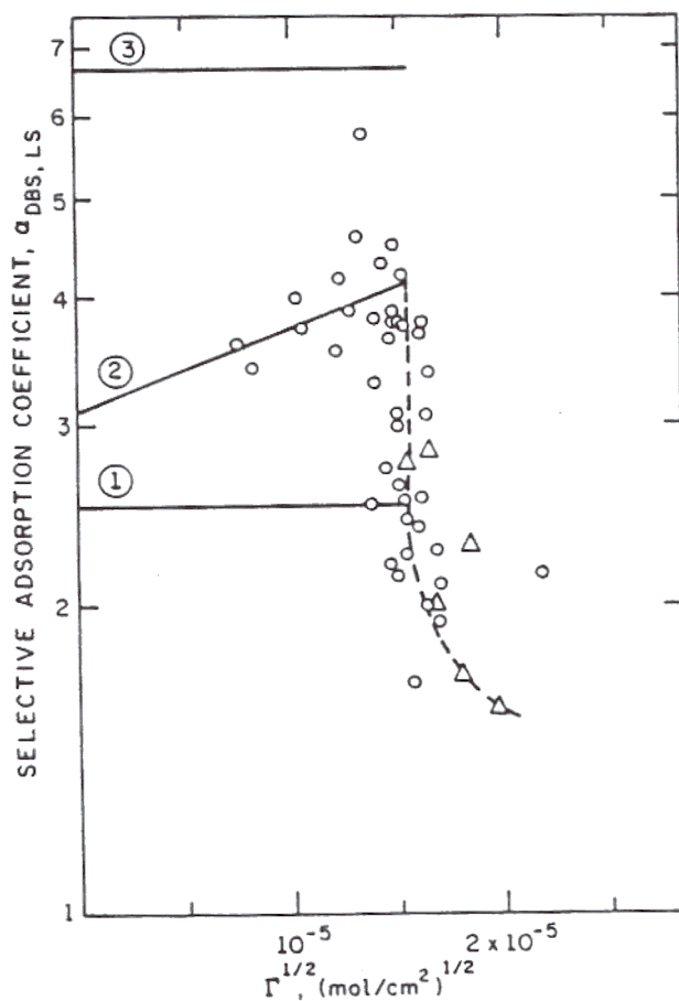
Figure 4. Adsorption coefficient of docetylbenzene sulfate (DBS) relative to that of lauryl sulfate (LS) as a function of total surface excess. (20) 1. Longmuir model (foaming experiment), 2. Long-chain ions model, 3. Longmuir model (surface tension).
