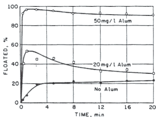
Figure 17. The effect of alum on the microflotation of B. cereus at pH 7 using 20 mg./liter lauric acid (58) .
