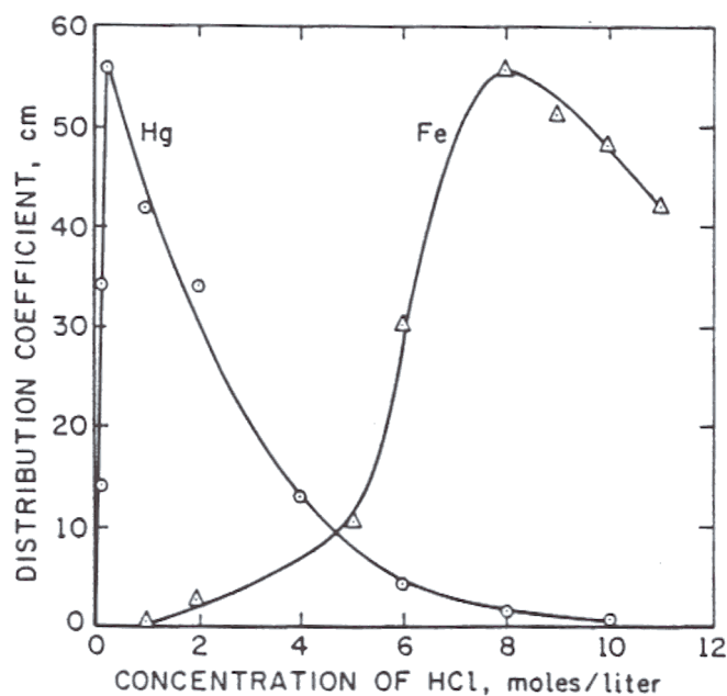
Figure 14. Distribution coefficients for Fe and Hg as a function of HCl concentration. a) Fe = 2 \times 10^{-3} H/l, surfactant (HDT) = 10^{-3} H/l b) Hg = 2 \times 10^{-7} H/l, surfactant (HDT) = 10^{-3} H/l
