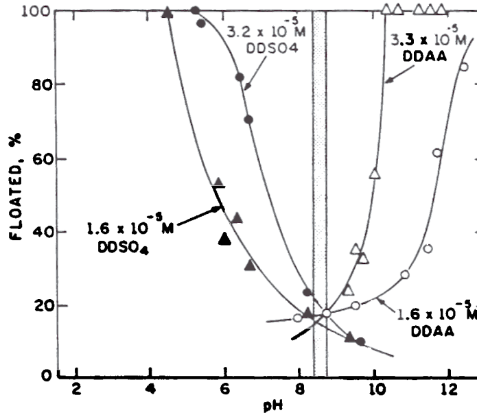
Figure 7. Flotation of calcite with dodecylammonium acetate (DDA) and sodium dodecylsulfate (DDSO 4 ) solutions (43) .
