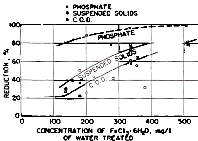
Figure 18. The effect of ferric chloride on the removal of phosphate and suspended matter (59) .
