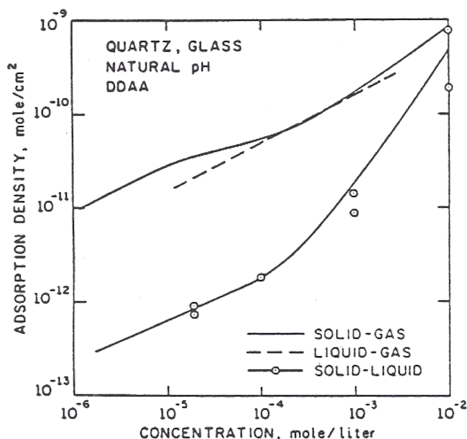
Figure 5. Adsorption density of dodecylammonium acetate at different interfaces (6) .
