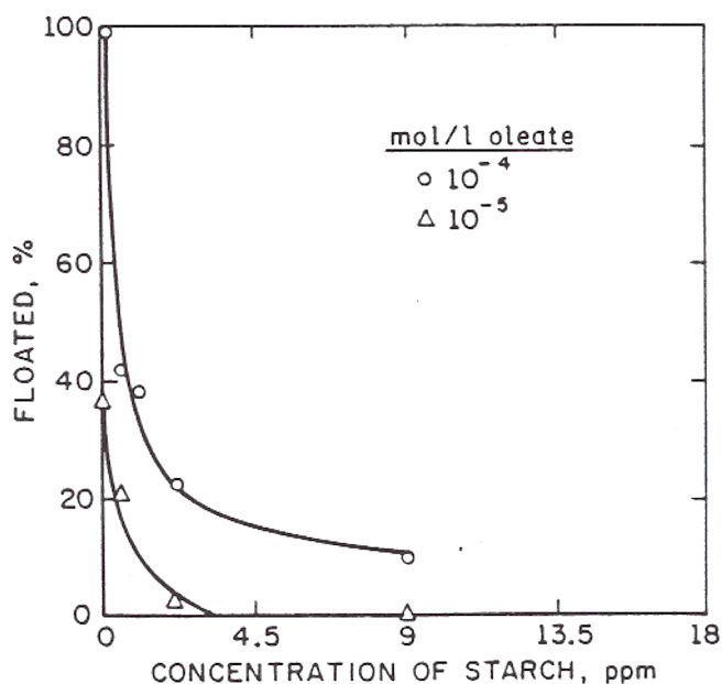
Figure 11. Percent of calcite floated as a function of starch in 10^{-4} mole/liter sodium oleate solutions (49) .
