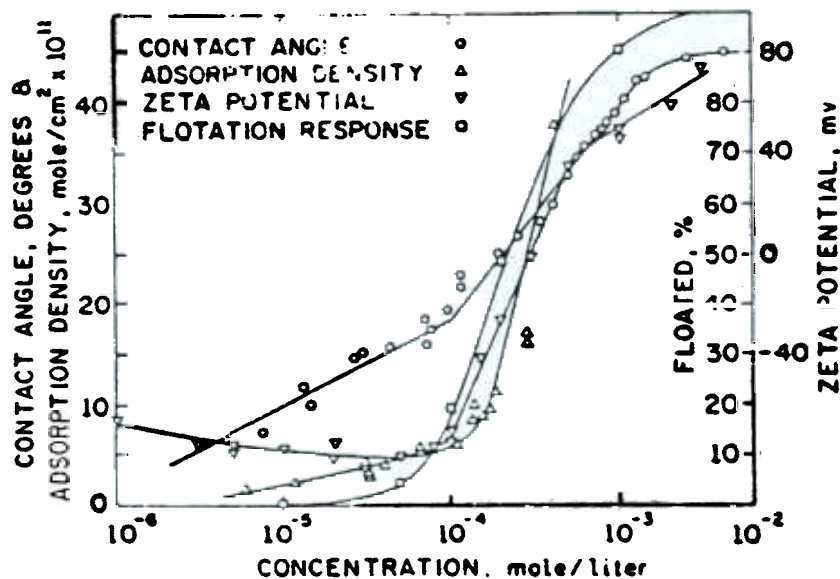
Figure 6. Correlation diagram of contact angle, adsorption density, flotation, and zeta potential for quartz as a function of dodecylammonium acetate concentration at pH 6 to 7, 20 to 25° C (21) .
